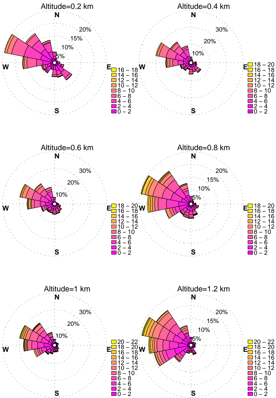
WINDROSES. PINEY RUN, MD WIND PROFILER. AUGUST, HOURS: 12 pm to 3 pm DATA: FROM 2010 to 2015
