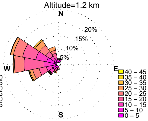
WINDROSES. PINEY RUN, MD WIND PROFILER. DECEMBER, HOURS: 12 am to 3 am DATA: FROM 2010 to 2015
