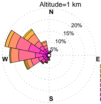
WINDROSES. PINEY RUN, MD WIND PROFILER. DECEMBER, HOURS: 12 am to 3 am DATA: FROM 2010 to 2015
