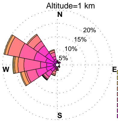
WINDROSES. PINEY RUN, MD WIND PROFILER. DECEMBER, HOURS: 12 pm to 3 pm DATA: FROM 2010 to 2015
