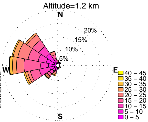
WINDROSES. PINEY RUN, MD WIND PROFILER. DECEMBER, HOURS: 12 pm to 3 pm DATA: FROM 2010 to 2015
