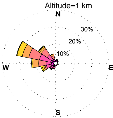
WINDROSES. PINEY RUN, MD WIND PROFILER. FEBRUARY, HOURS: 12 am to 3 am DATA: FROM 2010 to 2015
