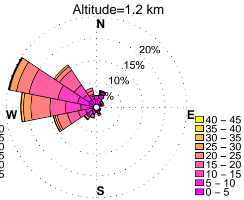
WINDROSES. PINEY RUN, MD WIND PROFILER. FEBRUARY, HOURS: 12 pm to 3 pm DATA: FROM 2010 to 2015
