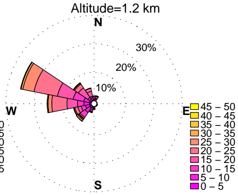
WINDROSES. PINEY RUN, MD WIND PROFILER. JANUARY, HOURS: 12 am to 3 am DATA: FROM 2010 to 2015
