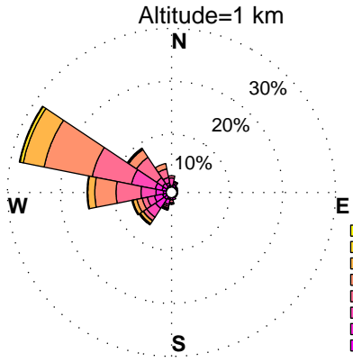
WINDROSES. PINEY RUN, MD WIND PROFILER. JANUARY, HOURS: 12 am to 3 am DATA: FROM 2010 to 2015
