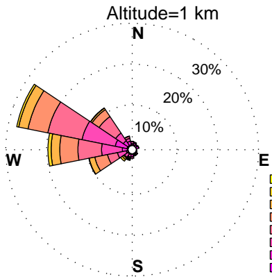
WINDROSES. PINEY RUN, MD WIND PROFILER. JANUARY, HOURS: 12 pm to 3 pm DATA: FROM 2010 to 2015
