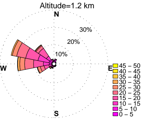
WINDROSES. PINEY RUN, MD WIND PROFILER. JANUARY, HOURS: 12 pm to 3 pm DATA: FROM 2010 to 2015
