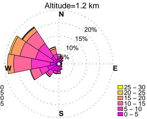
WINDROSES. PINEY RUN, MD WIND PROFILER. JULY, HOURS: 12 am to 3 am DATA: FROM 2010 to 2015
