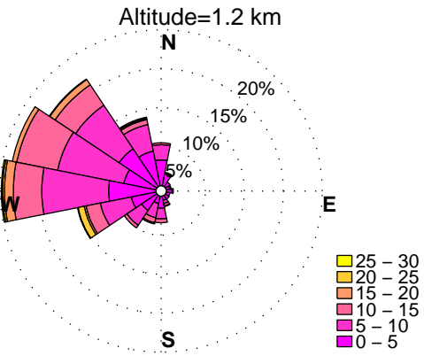
WINDROSES. PINEY RUN, MD WIND PROFILER. JULY, HOURS: 12 pm to 3 pm DATA: FROM 2010 to 2015
