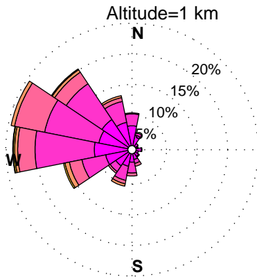
WINDROSES. PINEY RUN, MD WIND PROFILER. JULY, HOURS: 12 pm to 3 pm DATA: FROM 2010 to 2015
