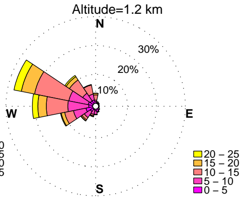
WINDROSES. PINEY RUN, MD WIND PROFILER. JUNE, HOURS: 12 am to 3 am DATA: FROM 2010 to 2015
