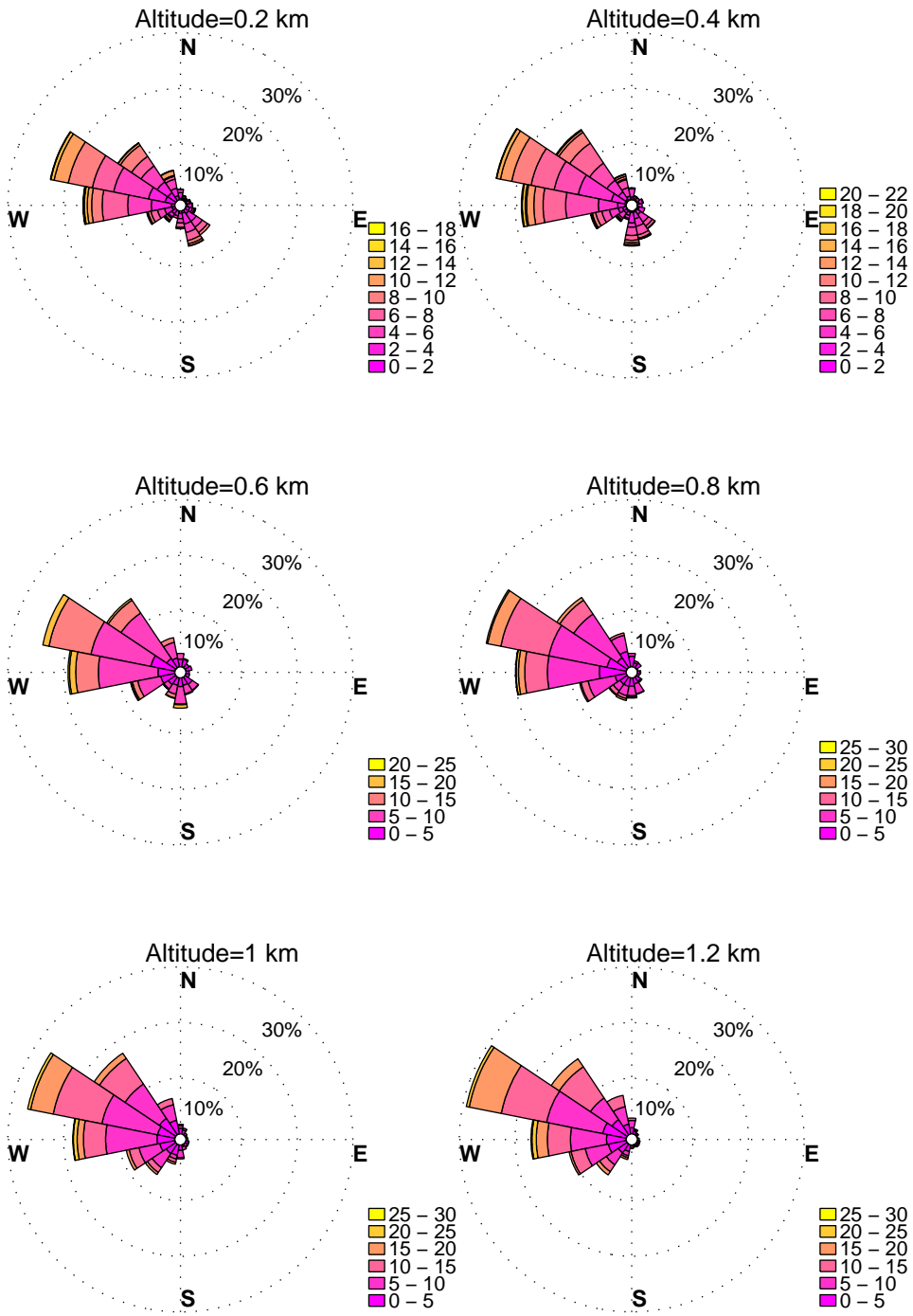
WINDROSES. PINEY RUN, MD WIND PROFILER. JUNE, HOURS: 12 pm to 3 pm DATA: FROM 2010 to 2015
