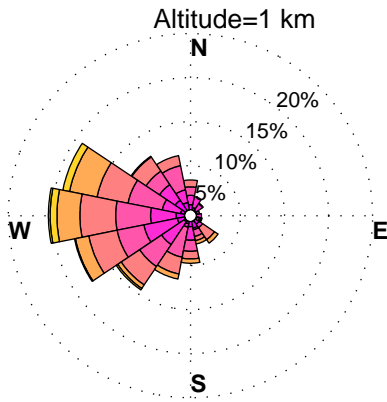
WINDROSES. PINEY RUN, MD WIND PROFILER. MAY, HOURS: 12 am to 3 am DATA: FROM 2010 to 2015
