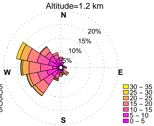
WINDROSES. PINEY RUN, MD WIND PROFILER. MAY, HOURS: 12 am to 3 am DATA: FROM 2010 to 2015
