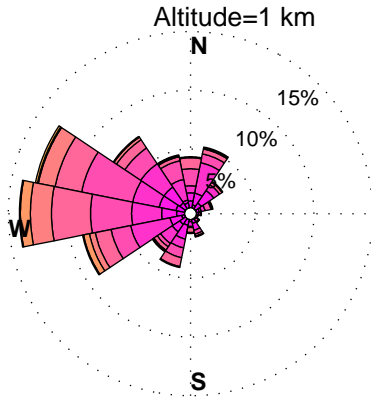
WINDROSES. PINEY RUN, MD WIND PROFILER. NOVEMBER, HOURS: 12 am to 3 am DATA: FROM 2010 to 2015
