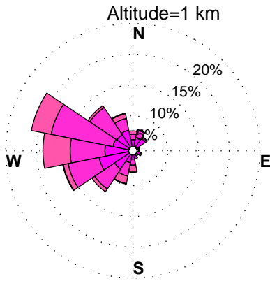
WINDROSES. PINEY RUN, MD WIND PROFILER. NOVEMBER, HOURS: 12 pm to 3 pm DATA: FROM 2010 to 2015
