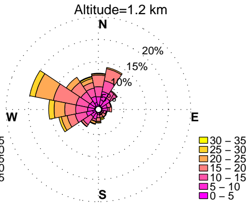
WINDROSES. PINEY RUN, MD WIND PROFILER. OCTOBER, HOURS: 12 am to 3 am DATA: FROM 2010 to 2015
