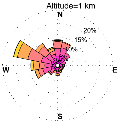
WINDROSES. PINEY RUN, MD WIND PROFILER. OCTOBER, HOURS: 12 am to 3 am DATA: FROM 2010 to 2015
