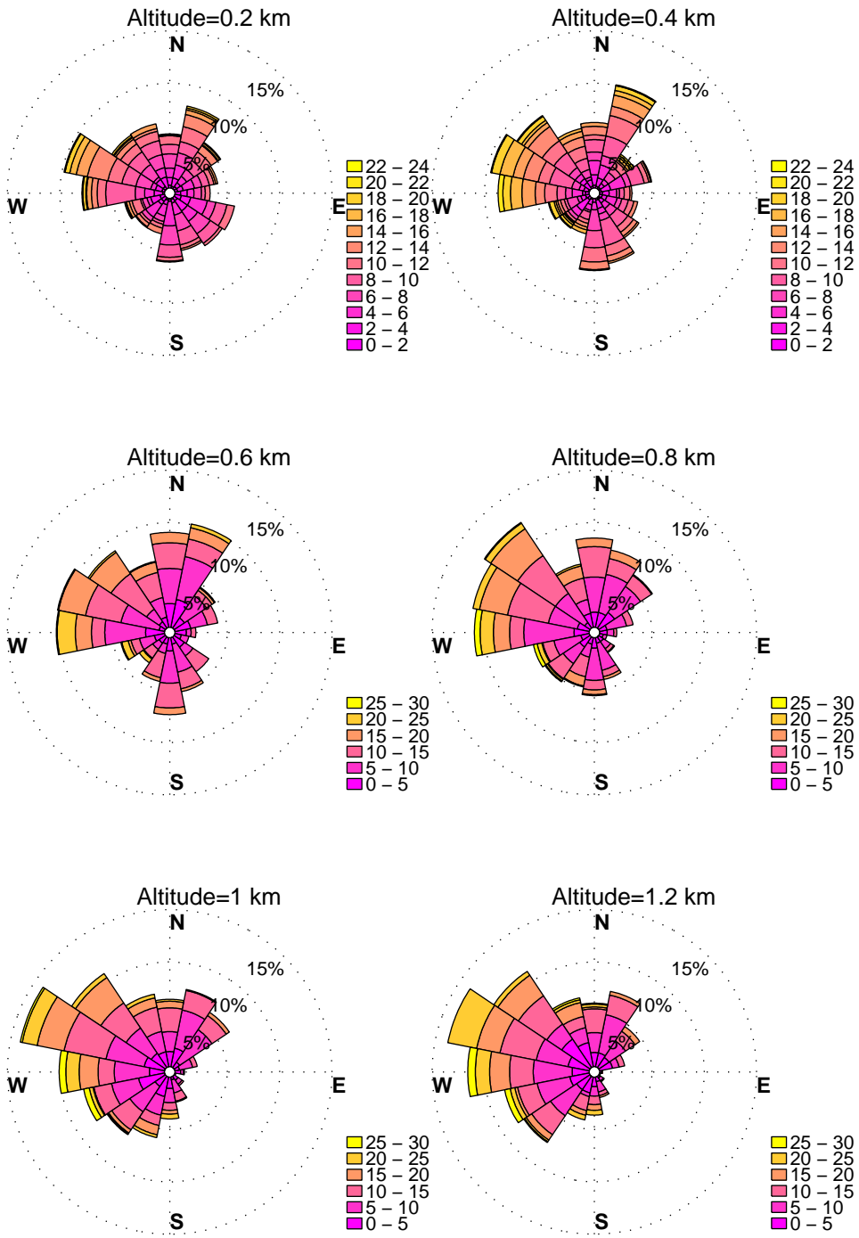
WINDROSES. PINEY RUN, MD WIND PROFILER. SEPTEMBER, HOURS: 12 am to 3 am DATA: FROM 2010 to 2015
