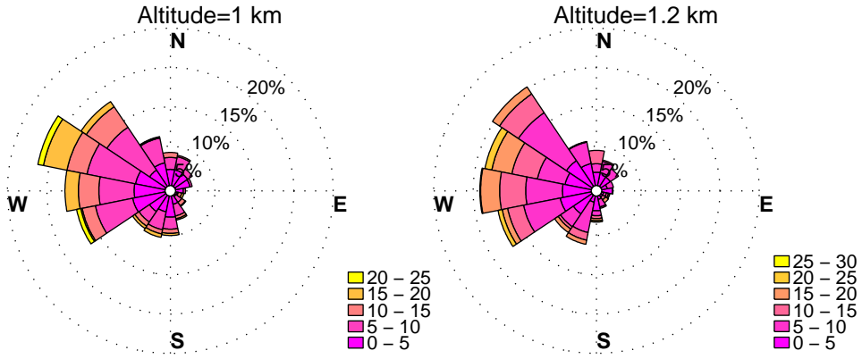
WINDROSES. PINEY RUN, MD WIND PROFILER. SEPTEMBER, HOURS: 12 pm to 3 pm DATA: FROM 2010 to 2015
