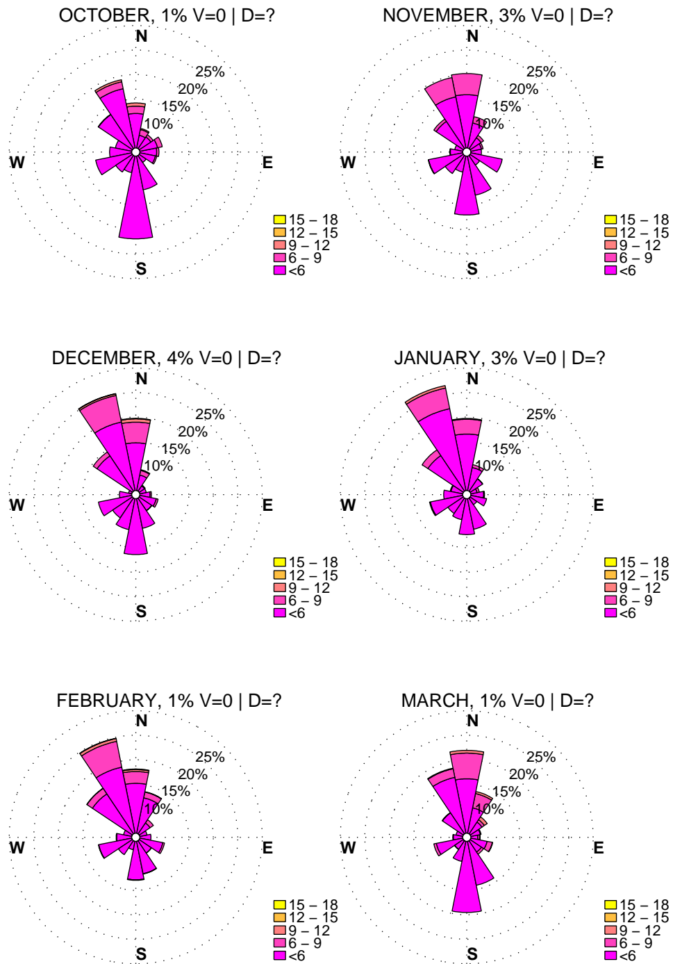
WINDROSES. BALTIMORE, MD. WINTER. HOURS: 12 to 16. Wind Speed in m/sec DATA: FROM 1/2010 to 12/2013.
