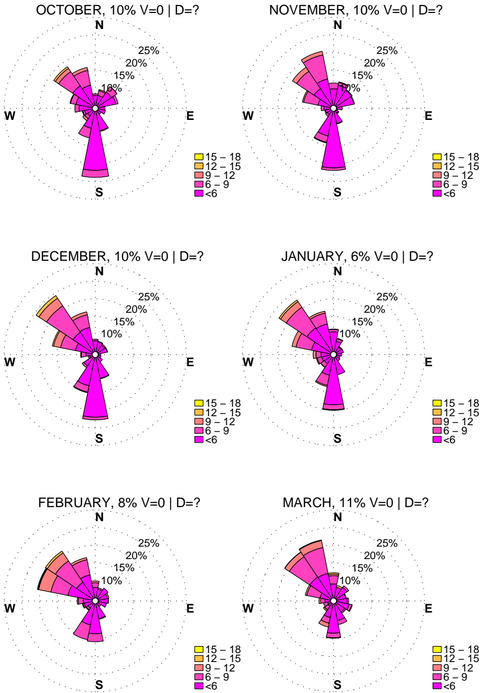
WINDROSES. MD AIRPORT: KDCA. WINTER. , HOURS: 12 to 16. Wind Speed in m/sec DATA: FROM 1/2010 to 12/2013.
