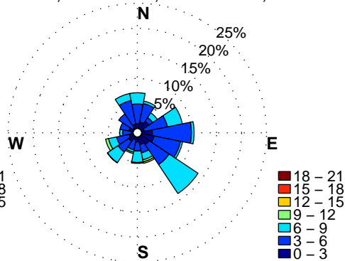
SEP, 54% Calm, <1% VarDir, n=730
