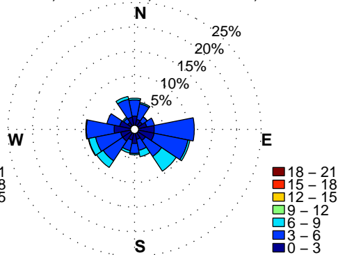
JUL, 50% Calm, <1% VarDir, n=920
