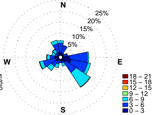
MAY, 49% Calm, <1% VarDir, n=840
