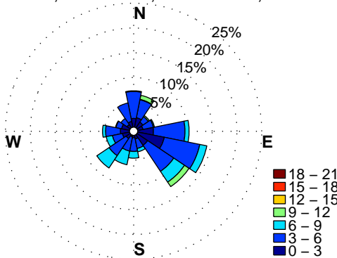
AUG, 50% Calm, <1% VarDir, n=907
