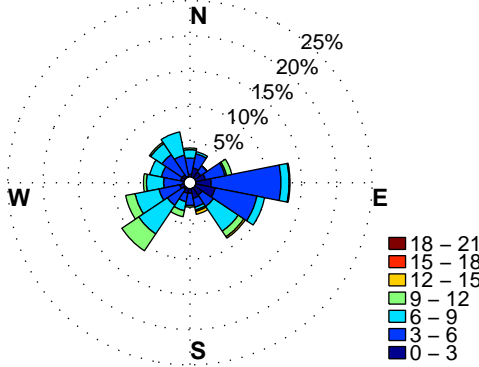
APR, 41% Calm, <1% VarDir, n=739
