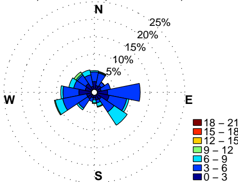
JUN, 51% Calm, <1% VarDir, n=875
