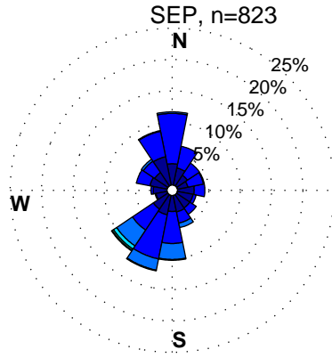
HU-BELTSVILLE, MD. WIND ROSES of HOURLY AVERAGES WARM SEASON MONTHS, HOURS: 12 to 16 Eastern Standard Time. Wind Speed: m/sec. Hourly data: 1/2010 – 8/2016.
