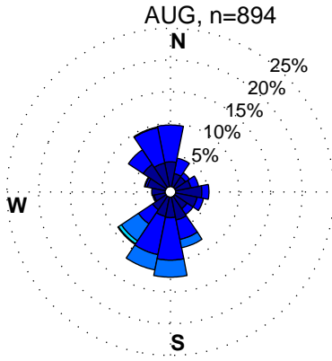
HU-BELTSVILLE, MD. WIND ROSES of HOURLY AVERAGES WARM SEASON MONTHS, HOURS: 12 to 16 Eastern Standard Time. Wind Speed: m/sec. Hourly data: 1/2010 – 8/2016.
