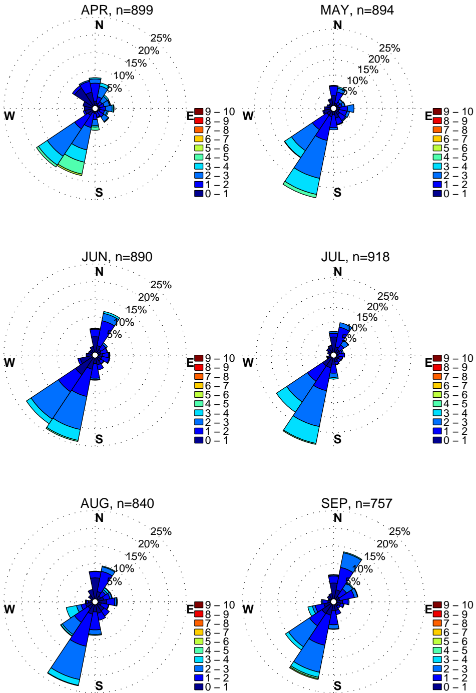
EDGEWOOD, MD. WIND ROSES of HOURLY AVERAGES WARM SEASON MONTHS, HOURS: 12 to 16 Eastern Standard Time. Wind Speed: m/sec. Hourly data: 1/2010 – 8/2016.
