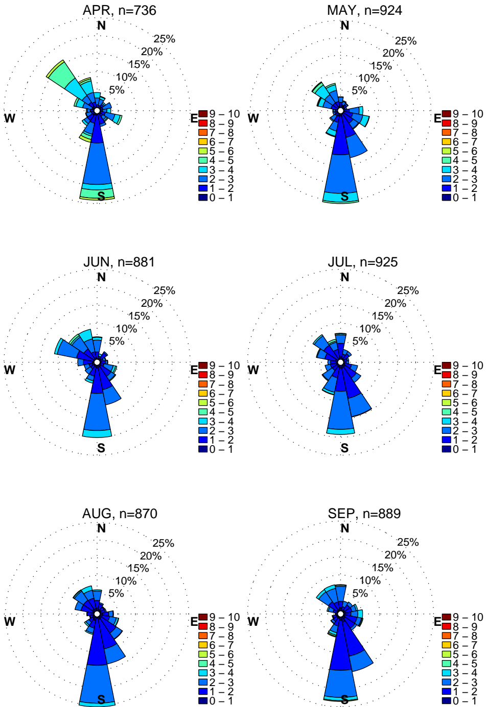
ESSEX, MD. WIND ROSES of HOURLY AVERAGES WARM SEASON MONTHS, HOURS: 12 to 16 Eastern Standard Time. Wind Speed: m/sec. Hourly data: 1/2010 – 8/2016.
