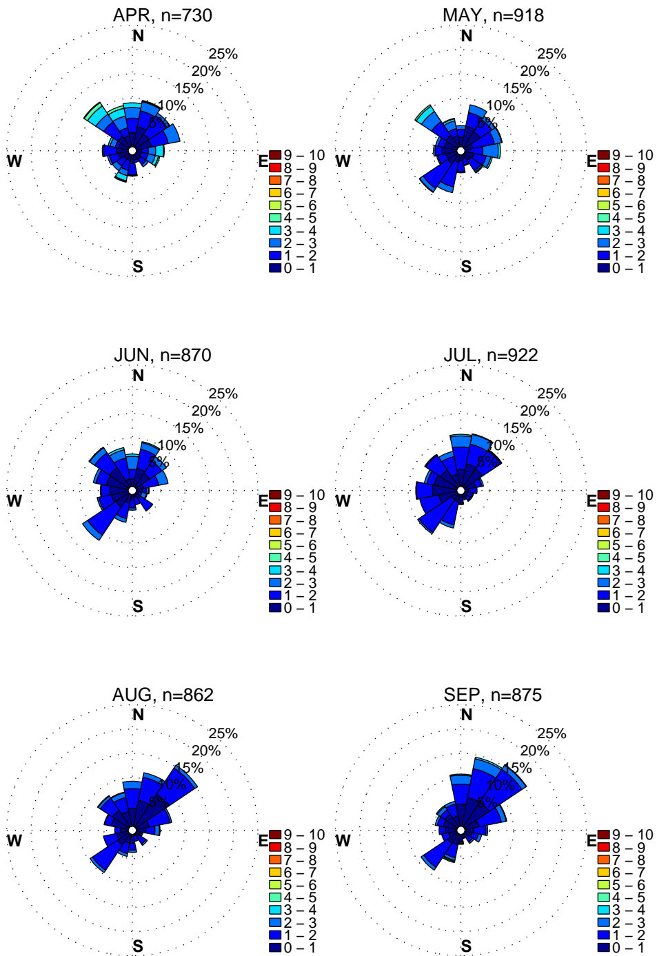
ESSEX, MD. WIND ROSES of HOURLY AVERAGES WARM SEASON MONTHS, HOURS: 4 to 8 Eastern Standard Time. Wind Speed: m/sec. Hourly data: 1/2010 – 8/2016.
