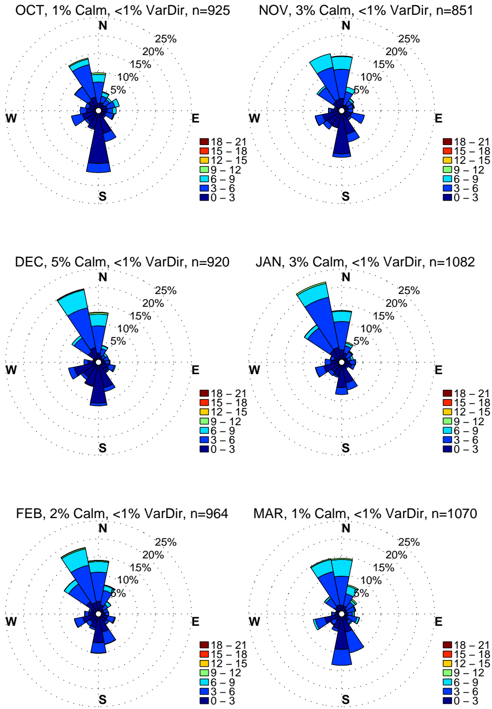
BALTIMORE CITY, MD WIND ROSES. COLD SEASON MONTHS, HOURS: 12 to 16 Eastern Standard Time. Wind Speed: m/sec. Hourly data: 1/2010 – 8/2016. Excluded: Calm & VarDir.
