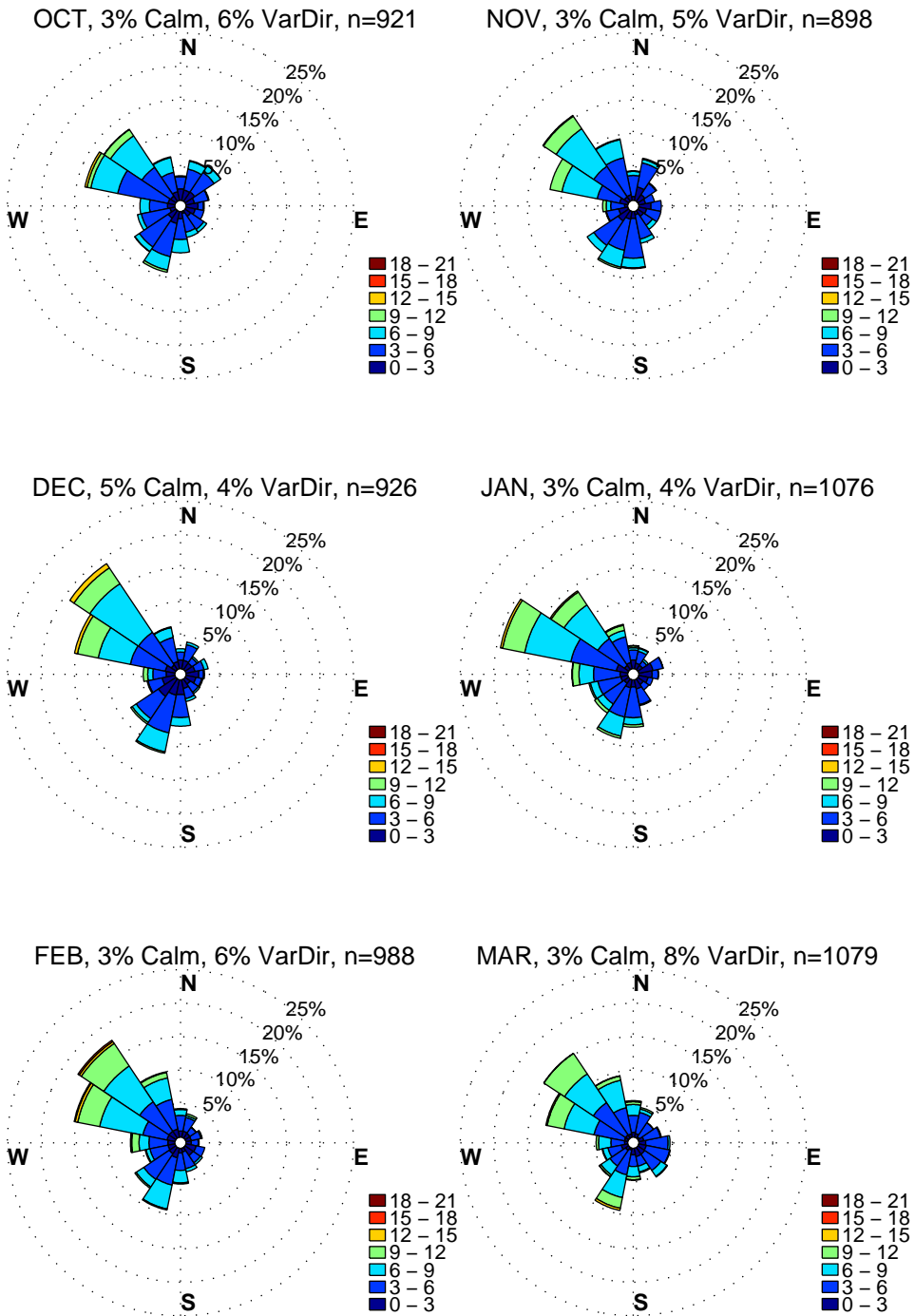
ANDREWS AIR FORCE BASE. WIND ROSES. COLD SEASON MONTHS, HOURS: 12 to 16 Eastern Standard Time. Wind Speed: m/sec. Hourly data: 1/2010 – 8/2016. Excluded: Calm & VarDir.
