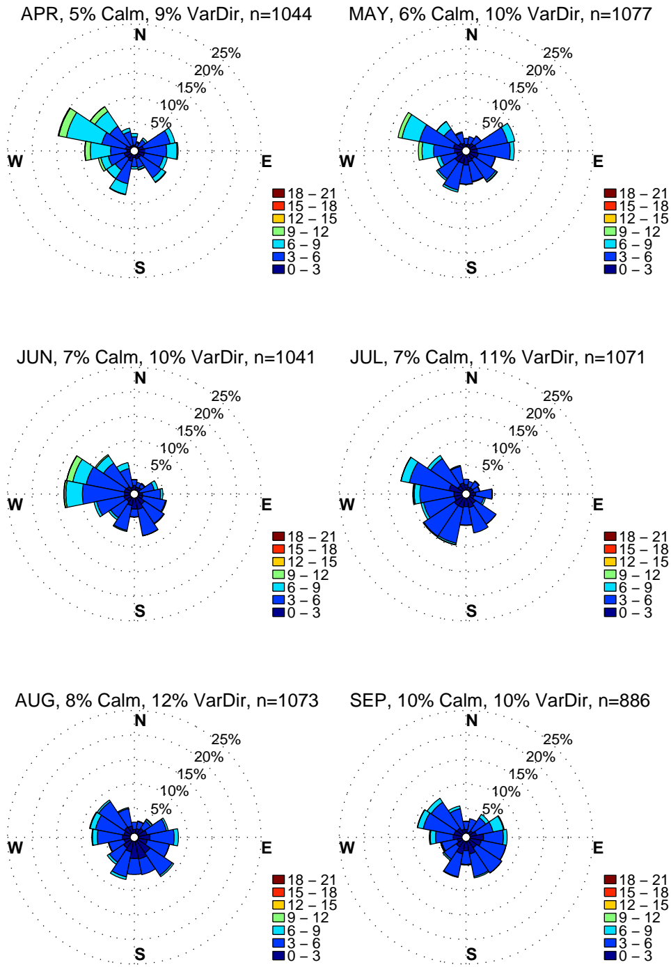
BALTIMORE WASHINGTON INT. AIRPORT. WIND ROSES. WARM SEASON MONTHS, HOURS: 12 to 16 Eastern Standard Time. Wind Speed: m/sec. Hourly data: 1/2010 – 8/2016. Excluded: Calm & VarDir.
