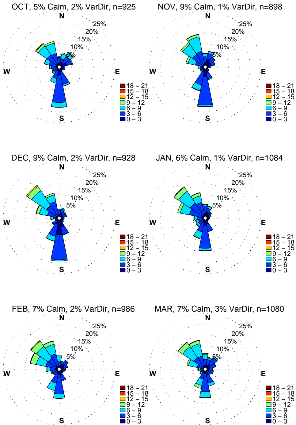
WASHINGTON NATIONAL AIRPORT. WIND ROSES. COLD SEASON MONTHS, HOURS: 12 to 16 Eastern Standard Time. Wind Speed: m/sec. Hourly data: 1/2010 – 8/2016. Excluded: Calm & VarDir.
