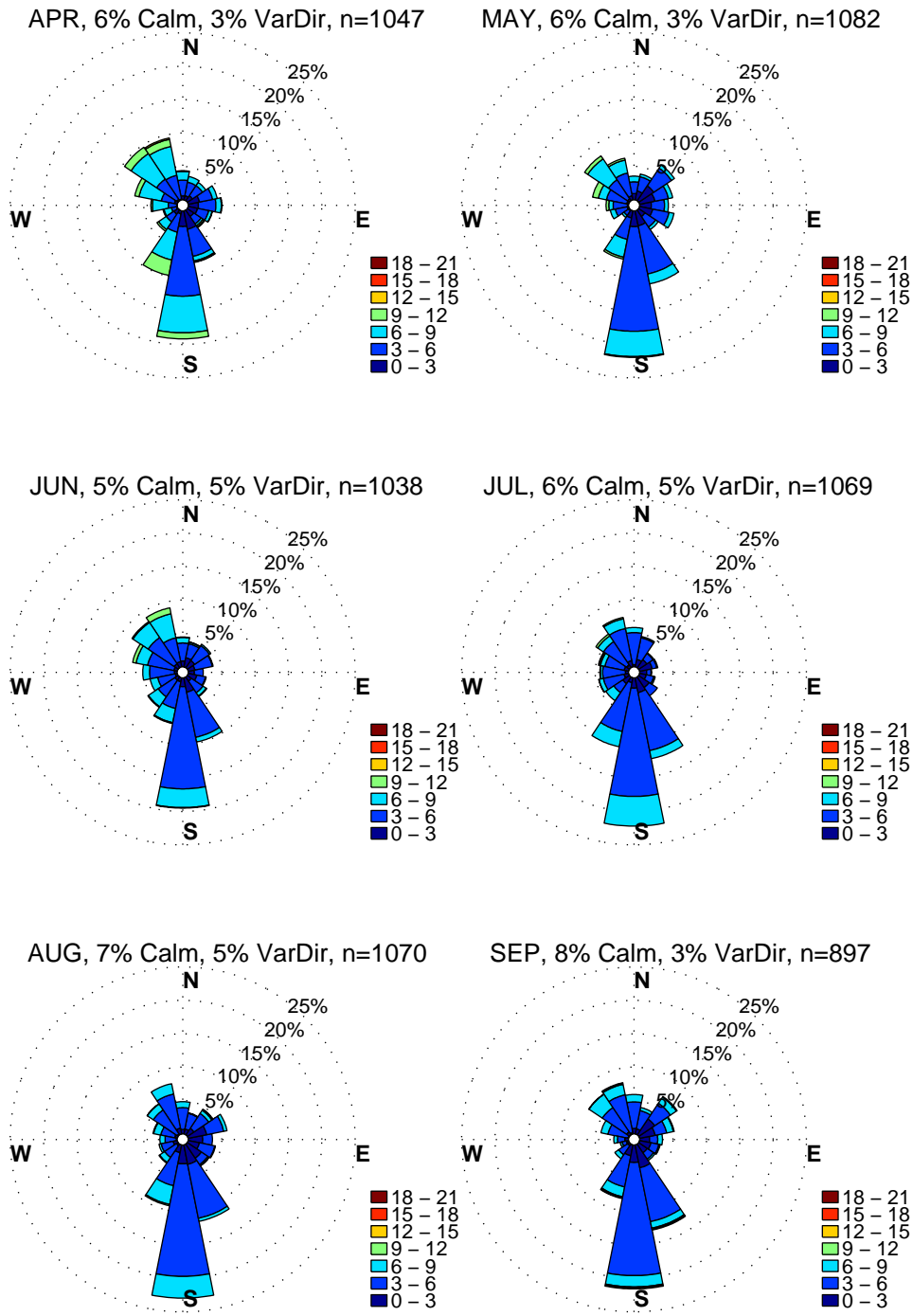
WASHINGTON NATIONAL AIRPORT. WIND ROSES. WARM SEASON MONTHS, HOURS: 12 to 16 Eastern Standard Time. Wind Speed: m/sec. Hourly data: 1/2010 – 8/2016. Excluded: Calm & VarDir.
