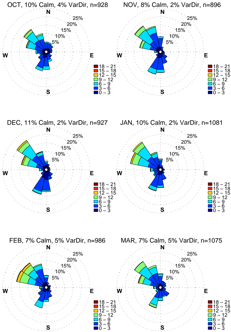
WASHINGTON DULLES INTERNATIONAL AIRPORT. WIND ROSES. COLD SEASON MONTHS, HOURS: 12 to 16 Eastern Standard Time. Wind Speed: m/sec. Hourly data: 1/2010 – 8/2016. Excluded: Calm & VarDir.
