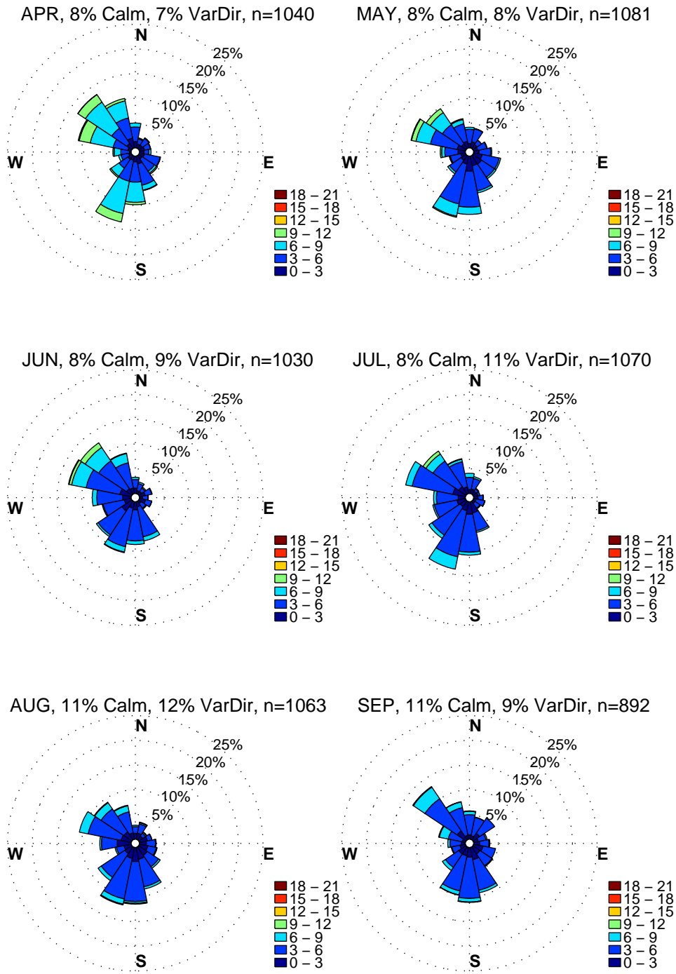
WASHINGTON DULLES INT. AIRPORT. WIND ROSES. WARM SEASON MONTHS, HOURS: 12 to 16 Eastern Standard Time. Wind Speed: m/sec. Hourly data: 1/2010 - 8/2016. Excluded: Calm & VarDir.
