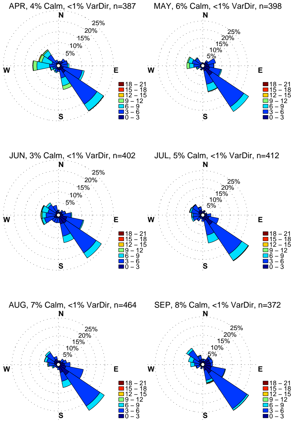
MARTIN STATE AIRPORT. WIND ROSES. WARM SEASON MONTHS, HOURS: 12 to 16 Eastern Standard Time. Wind Speed: m/sec. Hourly data: 1/2010 – 8/2016. Excluded: Calm & VarDir.
