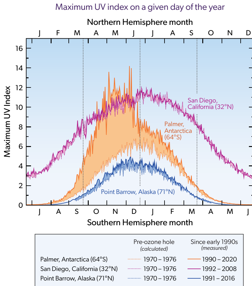
Figure Q16-2. Long-term changes in the UV Index (UVI), which is a measure of the erythemal radiation that reaches the surface. The figure shows the daily maximum UVI at three locations: San Diego, California; Point Barrow near Utqiagvik in northern Alaska; and Palmer Station in Antarctica. The daily maximum UVI is shown for two time periods: a more recent period corresponding to the availability of measurements starting in the early 1990s (solid lines, as indicated) and a pre-ozone hole time period of 1970–1976, computed using simulated total ozone values at the three locations for this time period. The shaded region for each measurement site represents the difference between the pre-ozone hole UVI and the observed UVI, starting with early 1990s data. The UVI observations from Palmer, Antarctica demonstrate the importance of ozone depletion on the amount of erythemal radiation reaching the surface. For 1990–2020, springtime values of the daily maximum UVI at Palmer equaled or exceeded those measured in spring at San Diego, which is located at a much lower latitude and, as a consequence, experienced much larger values of the daily maximum UVI than Palmer prior to the development of the ozone hole. The three thin vertical dotted lines show the dates of the spring equinox, the summer solstice, and the autumn equinox.
