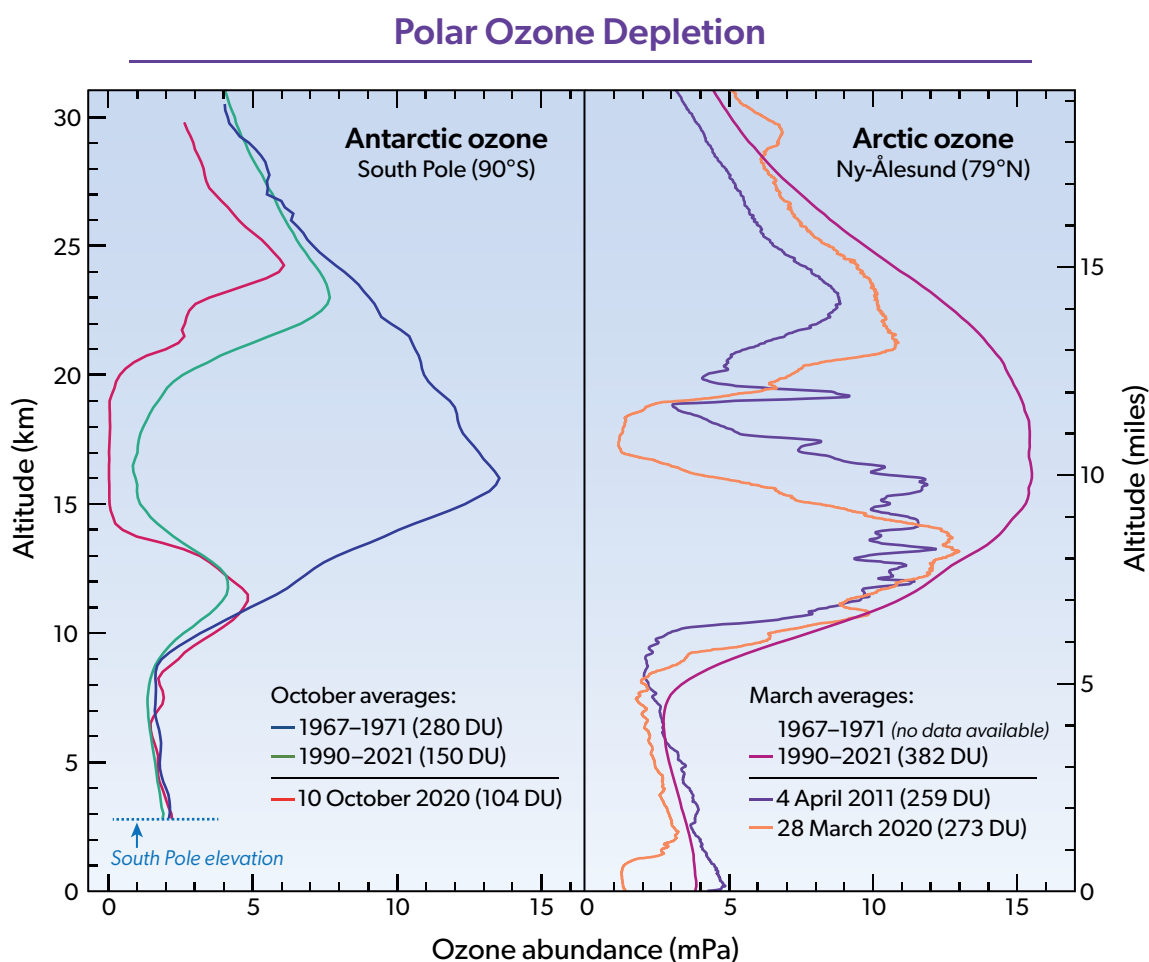
Figure Q11-3. Vertical distribution of Antarctic and Arctic ozone. At high latitudes during winter and spring, most stratospheric ozone resides between about 10 and 30 km (6 to 19 miles) above Earth's surface. Long-term observations of the ozone layer with balloon-borne ozone instruments also allow vertical profiles of ozone during winter to be compared between the Antarctic and Arctic regions. In the Antarctic at the South Pole (left panel), a normal ozone layer was observed to be present between 1967 and 1971. As shown here, ozone was almost completely destroyed between 14 and 20 km (9 to 12 miles) over the South Pole on 10 October 2020. Average October values of ozone in the last three decades (1990–2021) are 90% lower than pre-1971 values at the peak altitude of the ozone layer (16 km). For the Arctic, the average March profile for 1990–2021 as measured over the Ny-Ålesund research station is shown (right panel). No data from Ny-Ålesund are available for the 1967–1971 period. Some profiles reveal significant depletion, as shown here for 4 April 2011 and 28 March 2020. In such years, winter minimum temperatures are generally lower than normal, allowing for formation of PSCs and increases in ClO over longer periods of time. The number in parentheses for each profile is the total column ozone value in Dobson units (DU) (see box in Q4). Ozone abundances are shown here as the pressure of ozone at each altitude using the unit "milli-Pascals" (mPa) (100 million mPa = atmospheric sea-level pressure).
