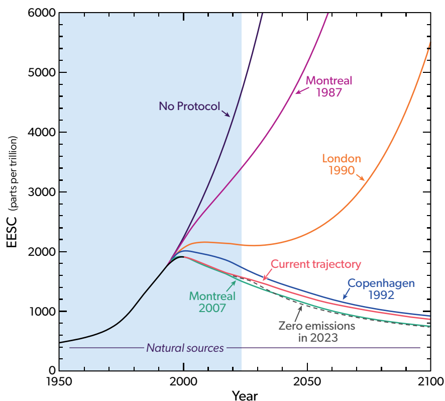
Figure Q14-1. Effect of the Montreal Protocol. The Montreal Protocol protects the ozone layer through control of the production and consumption of ozone-depleting substances (ODSs) by the world's nations. Equivalent effective stratospheric chlorine (EESC) is a quantity that represents the abundance of halogens available for ozone depletion in the stratosphere. Values of EESC are based upon either analysis of surface observations of ODSs (see Q15) or projections of future abundances of ODSs. Projections of EESC for the midlatitude lower stratosphere (about 19 km altitude) are shown separately for: no Protocol provisions; the provisions of the original 1987 Montreal Protocol and some of its subsequent amendments and adjustments as projected in 2007; the current trajectory for EESC (red solid curve); and for future EESC assuming zero emissions of ODSs starting in 2023 (black dashed curve). The city names and years indicate where and when changes to the original 1987 Protocol provisions were agreed upon (see Figure Q0-1). Without the Protocol, EESC values would have increased significantly in the 21st century, leading to large amounts of ozone depletion throughout the world, including over highly populated regions. Only with the Copenhagen (1992) and subsequent Amendments and Adjustments do projected EESC values show a long-term decrease. The EESC values from observations shown in Figure Q15-1 lie above the Montreal 2007 projection due mainly to the use
