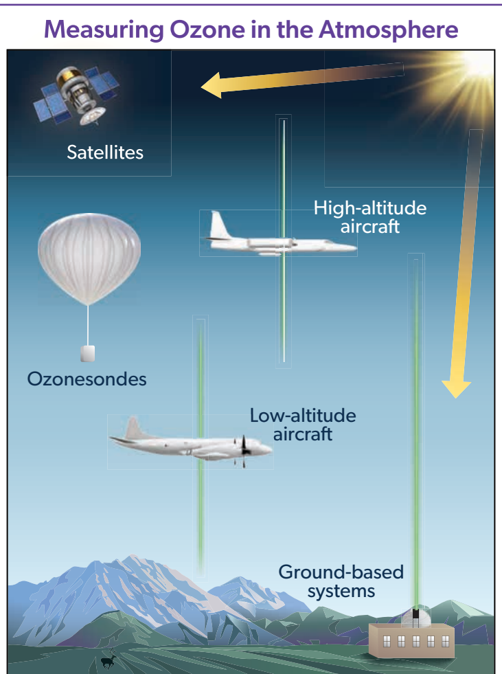
Figure Q4-1. Ozone measurements. Ozone is measured throughout the atmosphere with instruments on the ground, aircraft, high-altitude balloons, and satellites. Some instruments measure ozone locally in sampled air and others measure ozone remotely a considerable distance away from the instrument. Instruments use optical techniques with either the Sun (direct, reflected, or scattered radiation) or lasers (green lines) as light sources; detect the thermal emissions from ozone and other atmospheric molecules (not shown); or use chemical reactions that are unique to ozone (ozonesonde). At many locations over the globe, regular measurements are made to monitor ozone amounts and their variations over time.
