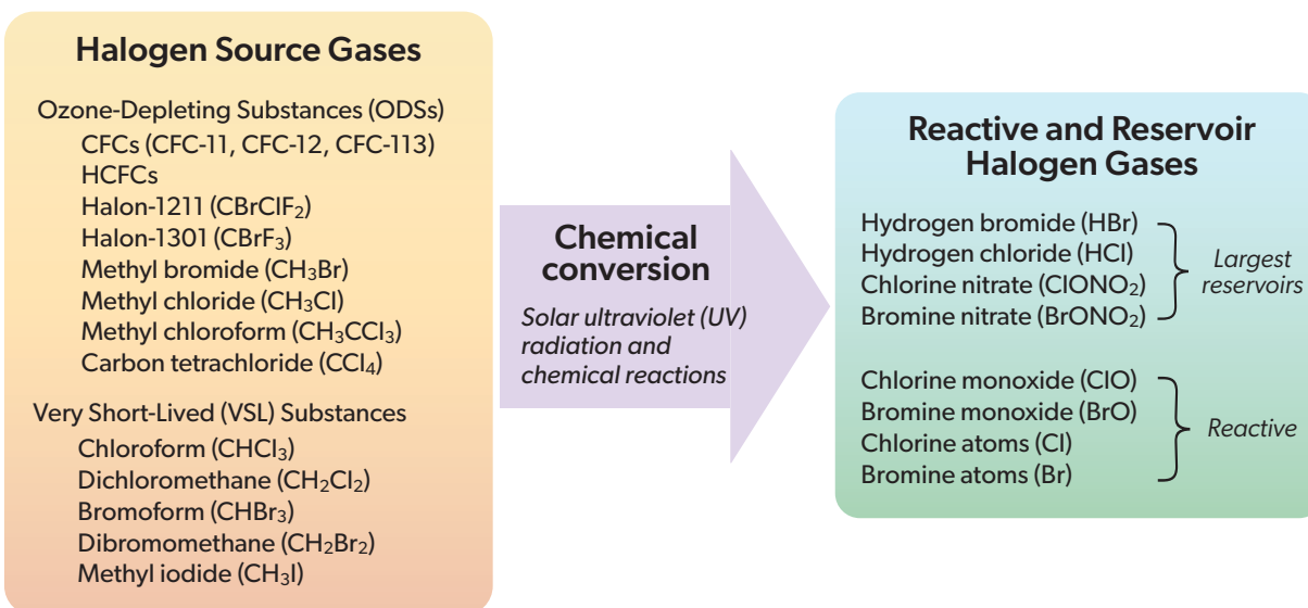
Figure Q7-1. Conversion of halogen source gases. Halogen source gases containing chlorine and bromine are chemically converted to reactive and reservoir halogen gases, primarily in the stratosphere. The conversion requires solar ultraviolet radiation and a few chemical reactions. The very short-lived substances undergo partial loss in the troposphere, so a smaller fraction of these gases reach the stratosphere compared to the other source gases. The gases produced by this chemical conversion can be grouped into the reservoir gases, which do not directly destroy ozone, and the reactive gases, which participate in ozone destruction cycles (see Q8). A principal reactive gas, ClO, is formed from the reservoir gases HCl and ClONO 2 by reactions that occur on the surfaces of liquid and solid polar stratospheric clouds (PSCs) (see Q9).
