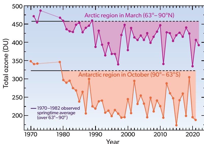
Figure Q11-1. Average total ozone in polar regions. Long-term changes in total ozone measured with satellite instruments are shown for the Antarctic and Arctic. The measurements are averaged over latitudes poleward of 63° for March (in the Arctic) and for October (in the Antarctic) and displayed as Dobson units (DU) (see box in Q4). The reference values (black lines) are averages of springtime total ozone from observations acquired between 1970 and 1982. After 1982, significant ozone depletion is found in most years in the Arctic and all years in the Antarctic. The largest average depletions have occurred in the Antarctic since 1990. The ozone changes arise from a combination of chemical destruction and natural variations in meteorological conditions that influence the year-to-year values of ozone, particularly in the Arctic. The year-to-year variation in Antarctic total ozone has increased since 2000.
