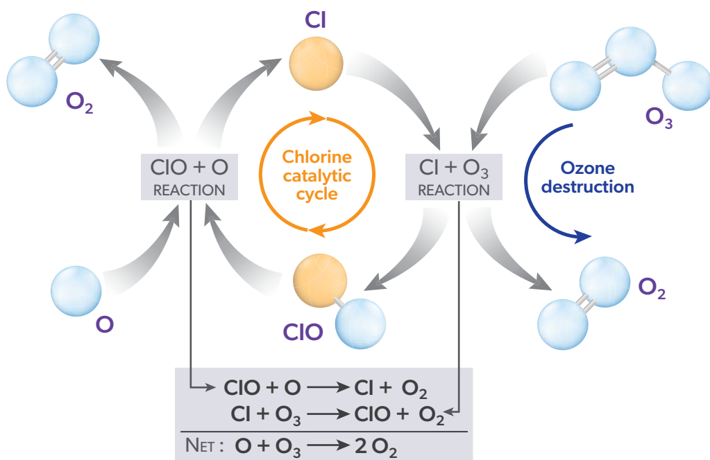
Figure Q8-1. Ozone destruction Cycle 1. The destruction of ozone in Cycle 1 involves two separate chemical reactions. The cycle can be considered to begin with either ClO or Cl. When starting with ClO, the first reaction is ClO with O to form Cl and O 2 . Then, Cl reacts with O 3 and reforms ClO, consuming O 3 in the process and forming another O 2 . The net or overall reaction is that of atomic oxygen (O) with ozone (O 3 ), forming two oxygen molecules (O 2 ). The cycle then begins again with another reaction of ClO with O. Chlorine is considered a catalyst for ozone destruction because Cl and ClO are reformed each time the reaction cycle is completed, and hence available for further destruction of ozone. Atomic oxygen is formed when solar ultraviolet (UV) radiation reacts with O 3 and O 2 molecules (see Figure Q1-3). Cycle 1 is most important in the stratosphere at tropical and middle latitudes, where solar UV radiation is most intense.
