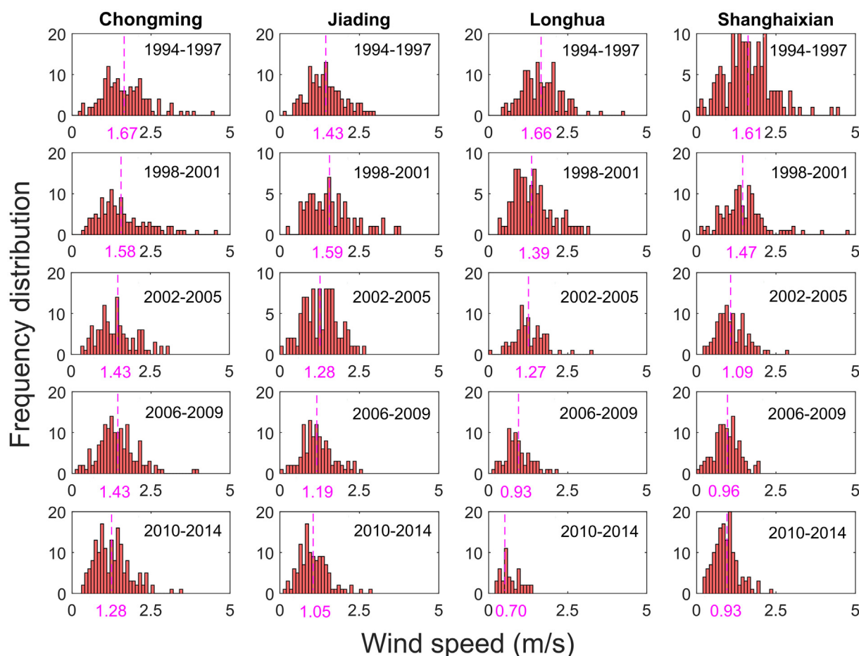
Fig. 4. Histograms of the marine wind speed of SLB in summer from 1994 to 2014 at other four sites in Shanghai: (a) Chongming, (b) Jiading, (c) Longhua, (d) Shanghai Xian. The pink lines represent the mean wind speed values for each time period. (For interpretation of the references to colour in this figure legend, the reader is referred to the web version of this article.)
