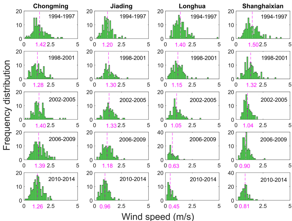
Fig. 5. Histograms of the land wind speed of SLB in summer from 1994 to 2014 at other four sites in Shanghai: (a) Chongming, (b) Jiading, (c) Longhua, (d) Shanghai Xian. The pink lines represent the mean wind speed values for each time period. (For interpretation of the references to colour in this figure legend, the reader is referred to the web version of this article.)
