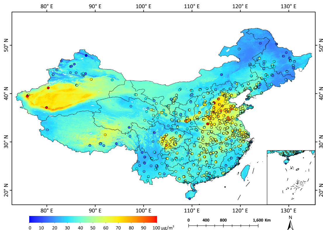
Fig. 8. Spatial distributions of satellite-estimated ( 0.01^\circ \times 0.01^\circ grid, background shading) and ground-measured (colored dots) PM 2.5 concentrations in 2016 across China.
