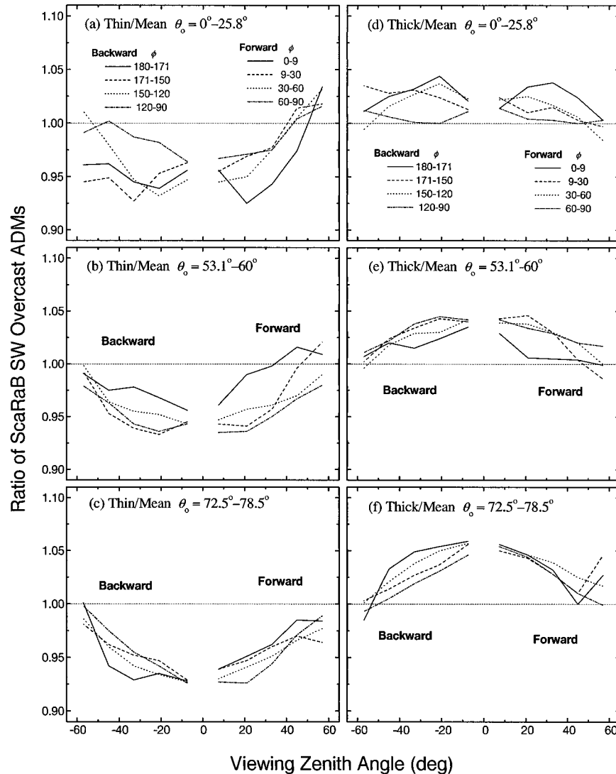
FIG. 6. Ratios of the ScaRaB thin to mean (left panels) and thick to mean (right panels) SW overcast ADMs for three SZA bins. Forward scattering denoted by positive VZAs for RAAs 0^{\circ} – 90^{\circ} ; backward scattering denoted by negative VZAs for RAAs 90^{\circ} – 180^{\circ} .
